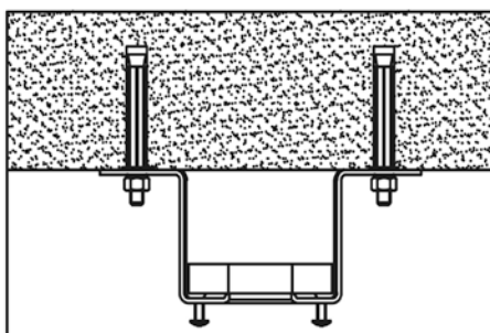
1-CEILING-MOUNT BRACKET
